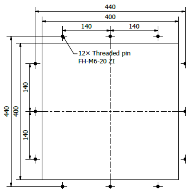
Fig. 3. Mounting dimensions in [mm]
