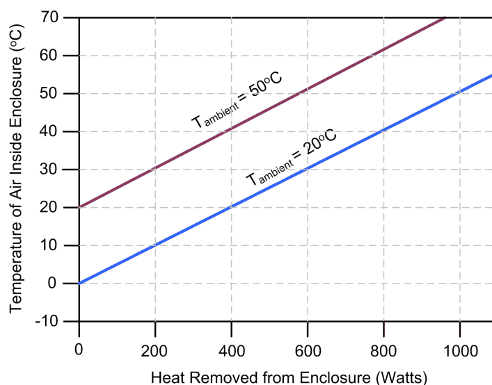
Fig. 1. MMB-TEC-900 performance lines
