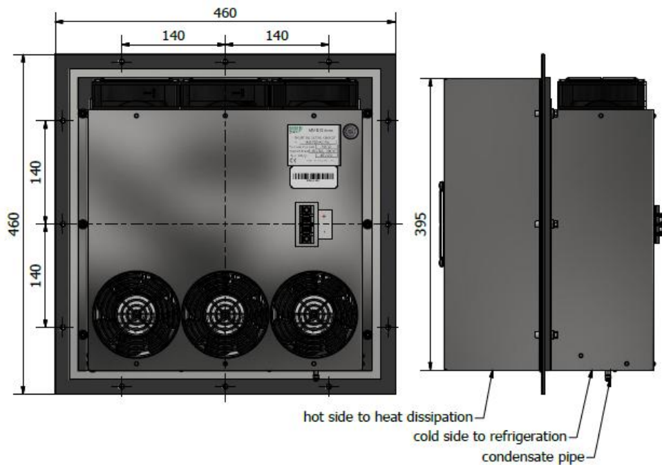
Fig. 2. MMB-TEC-900 dimensions in [mm]
